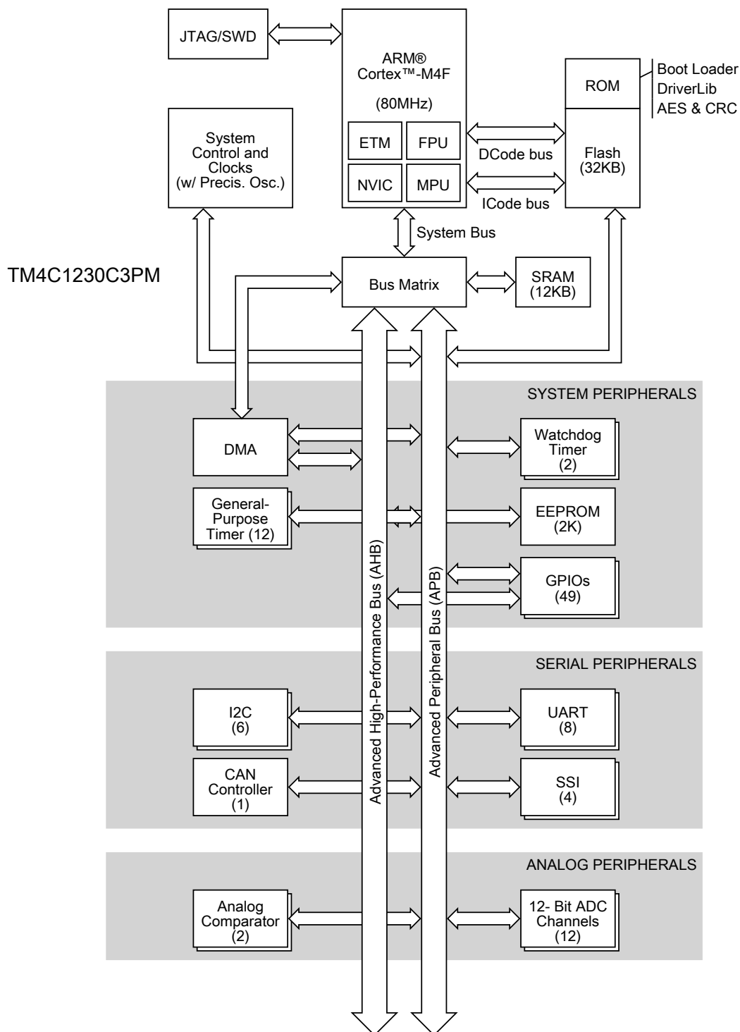
Figure 1-2. Tiva TM4C1230C3PM Microcontroller High-Level Block Diagram
